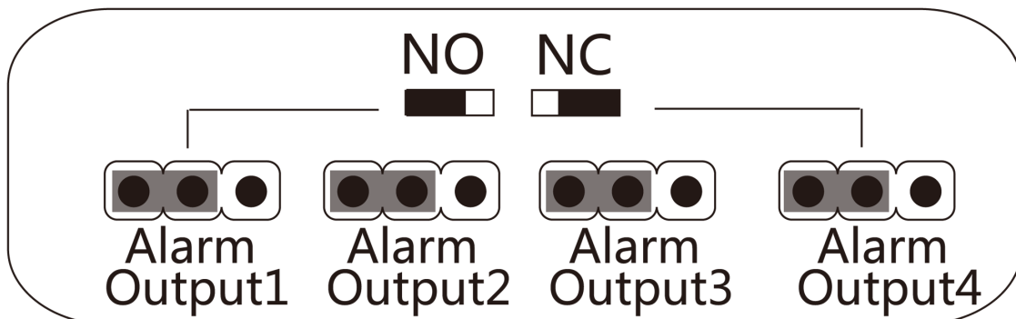
Figure 6-5 NO Status
