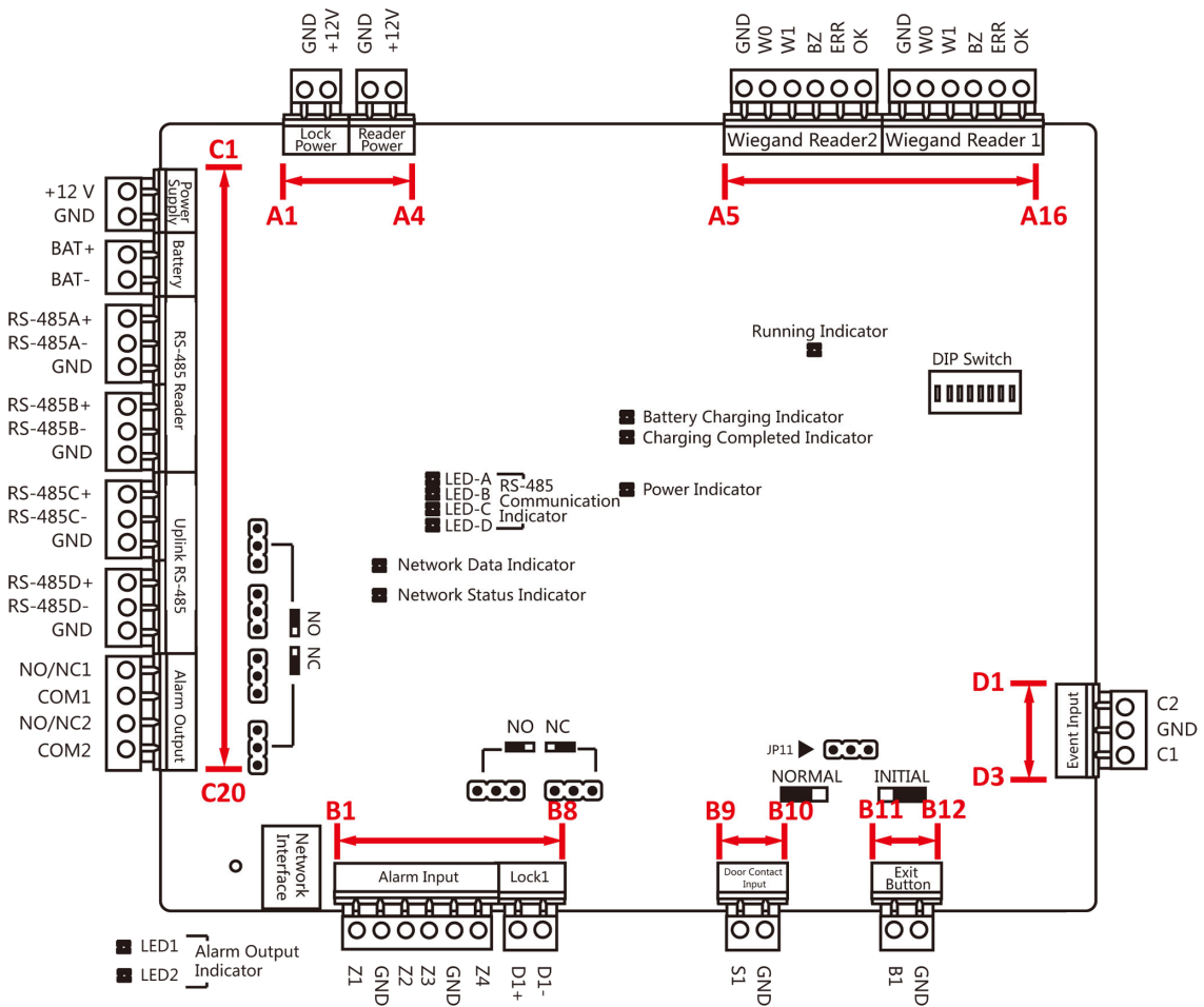
Figure 4-1 Single-Door Access Controller Main Board
