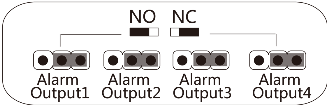
Figure 6-6 NC Status
