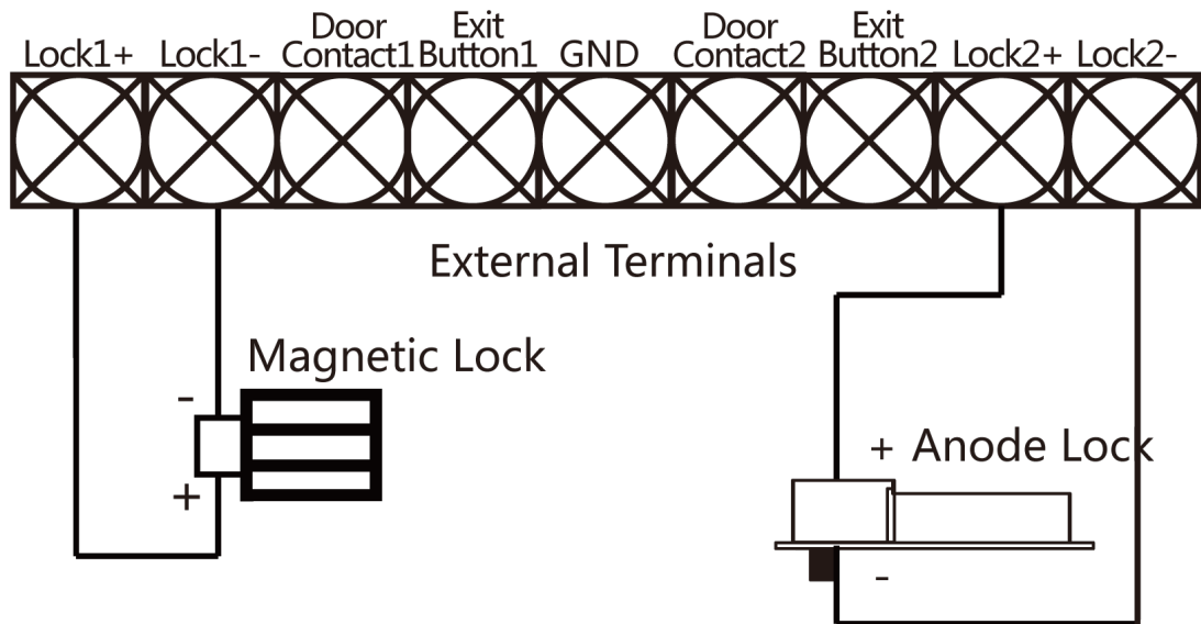
Figure 5-7 Wiring Diagram of Anode Lock
